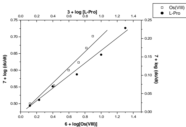
Fig. 4. Plot between rate \log[Os(VIII)] vs. \log(dc/dt) and \log[L-Pro] vs. \log(dc/dt) for oxidation of L-Pro at 308 K
