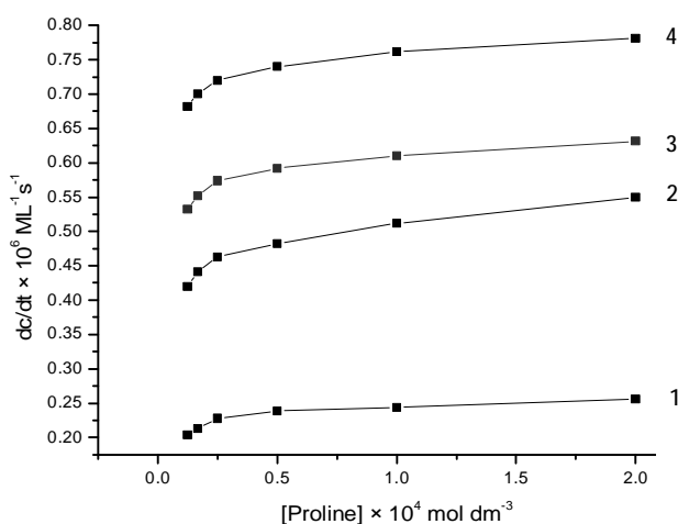
Fig. 3. Plot between rate of reaction (-dc/dt)\cdot 10^6 vs. [L-proline] \cdot 10^4 on the reaction rate at different temperatures (K): 303 (1), 308 (2), 313 (3) and 318 (4). [Os(VIII)] = 26.25\cdot 10^{-5} M, [Hg(OAc) 2 ] = 1.25\cdot 10^{-3} M, [Oxidant (NaIO 4 )] = 1.00\cdot 10^{-3} M, [NaOH] = 1.00\cdot 10^{-3} M
