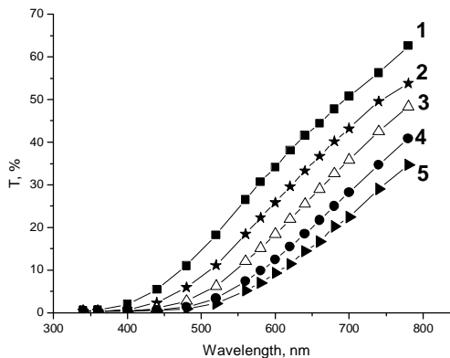
Fig. 4. Dependence of light transmittance of hydrogel samples filled with nanoparticles with average radius of 50 nm on the wavelength. The concentration of nanoparticles (wt% related to the amount of hydrogel) corresponds to (wt %): 0.11 (1); 0.15 (2); 0.21 (3); 0.26 (4) and 0.29 (5)
