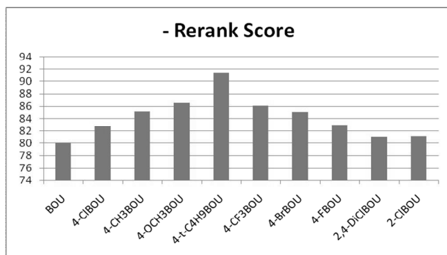
Fig. 2. RS values of 1-(benzoyloxy)urea and its derivatives
