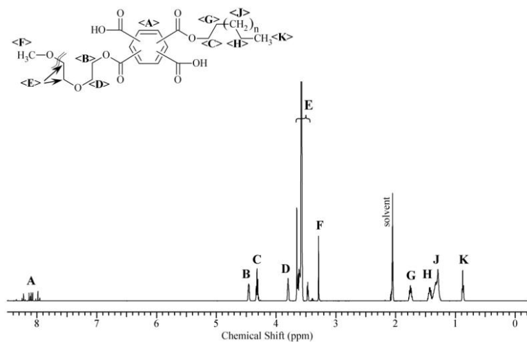
Fig. 7. Spectrum ^1\text{H} NMR of MPEG550-PMA-Alc (Alc = octyl). 7.90–8.50 (A, 2H); 4.40–4.45 (B, 2H); 4.29–4.33 (C, 2H); 3.80 (D, 2H); 3.45–3.70 (E, 44H); 3.27 (F, 3H); 1.70–1.78 (G, 2H); 1.38–1.47 (H, 2H); 1.27–1.37 (J, 2H); 0.85–0.95 (K, 3H); ( n = 4 )
