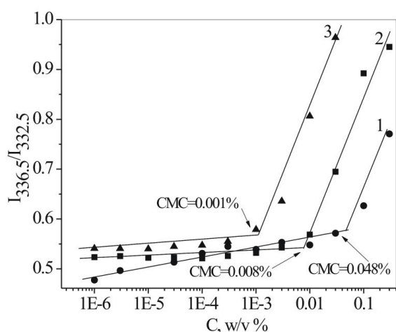
Fig. 10. The intensity ratio I_{336.5}/I_{332.5} of the excitation spectra of pyrene in OEPA solutions vs. OEPA concentration to determine CMC: MPEG550-PMDA-Oct (1); MPEG550-PMDA-Cet (2) and MPEG550-PMDA-Chol (3)
