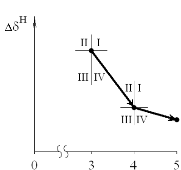
Fig. 3. Plot of the type 3 ( N-(o-m) > 0 and N-(m-p) > 0 )
