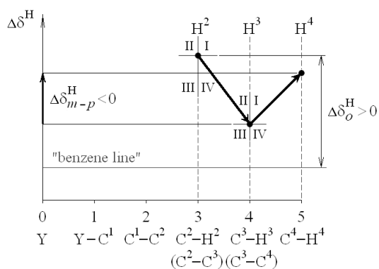
Fig. 2. Plot of the type 2 N-(o-m) > 0, N-(m-p) < 0
