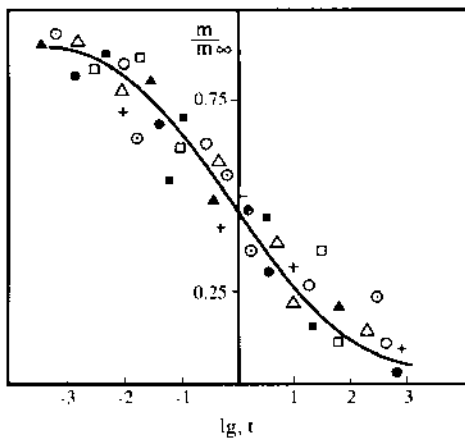
Fig. 8. Generalized kinetic curve of Aspergillus niger biomass inhibited growth in the presence of different biocides: ○ - merthiolate; ▲ - nyctedine; Δ - alkyl benzyl dimethylammonium chloride; ■ - CuSO 4 ; □ - oxydiphenyl-phenol; ● - N -paratolylmaleimide; + - ionol; o - phlamale(bis(0-1-chlortribrom-isopropyl)-trichlor-2-brompropylphosphonate)
