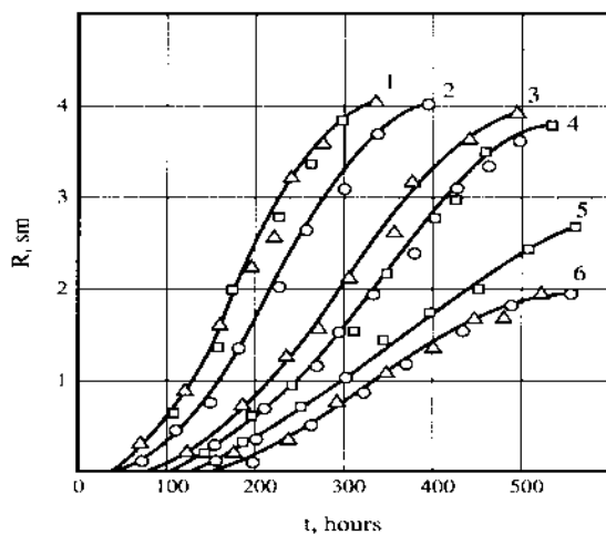
Fig. 4. Inhibition of the colony growth of different microscopic fungi, Aspergillus niger (1, 2), Trichoderma viride (3, 4), and Penicillium cyclopium (5, 6), on the agar nutrient of Chapect-Dox in the presence of the stabilizer biocide ionol (mg/l): \square - 2.5; \circ - 5 \cdot 10^4 ; \Delta - 7.5 \cdot 10^4
