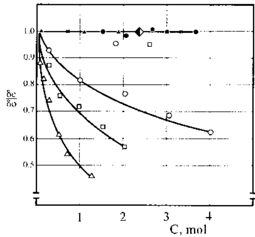
Fig. 13. Reduced elasticity of PMMA samples on elongation in acid solutions and water vs acid concentration: (o) acetic, (□) propionic, (□) butyric oil, (Δ) wine, (■) citric, (▲) oxalate, (x) amber and (◆) fumaric. Rate of elongation: 0.01 \text{ min}^{-1}
