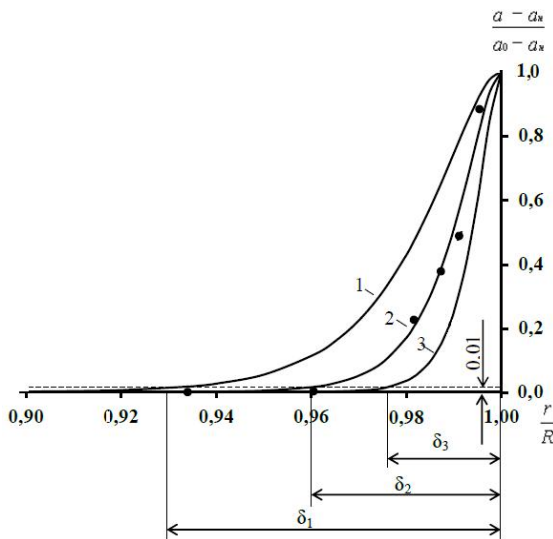
Fig. 3. The comparison of calculation and experimental types of concentration distribution of camphor: m = 70 , \delta_1 = 17.6 \cdot 10^{-6}\text{ m} (1); m = 120 , \delta_2 = 10.4 \cdot 10^{-6}\text{ m} (2) and m = 200 , \delta_3 = 7.2 \cdot 10^{-6}\text{ m} (3). C_i = 10\% ; t = 323\text{ K} ; \tau = 3600\text{ s}
